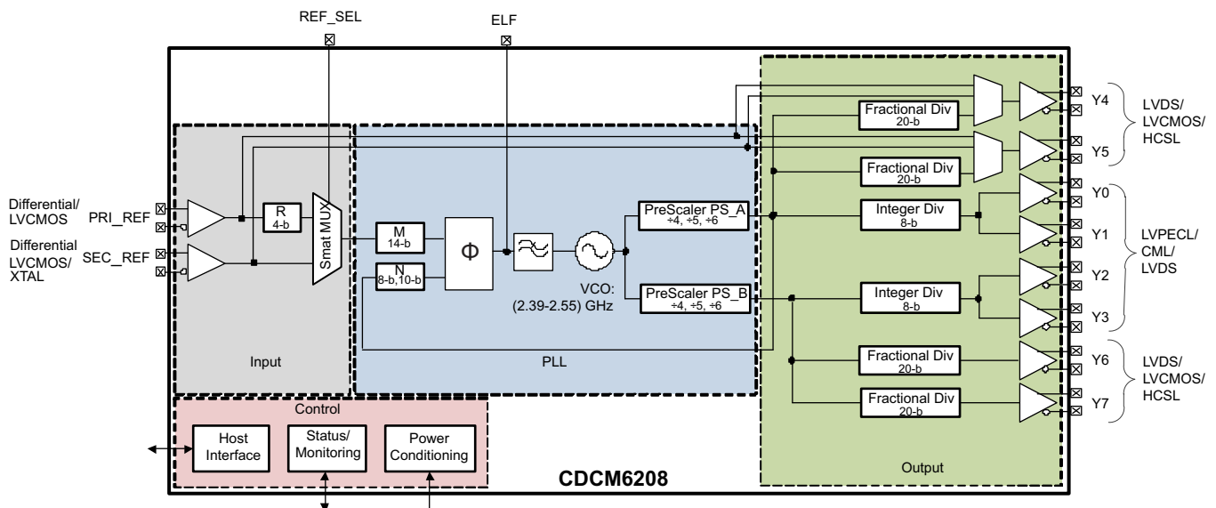
Figure 26. High-Level Block Diagram of CDCM6208V2G
