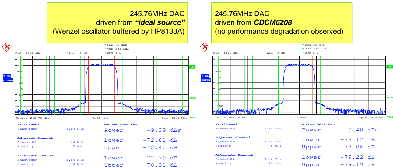
Figure 54. DAC Driven by Lab Source and CDCM6208V2G in Comparison (Performance Identical)
