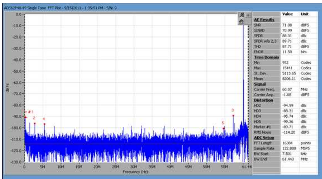
Figure 53. IF = 60 MHz Fclk = 122.88 MHz CDCM6208V2G driving ADC
