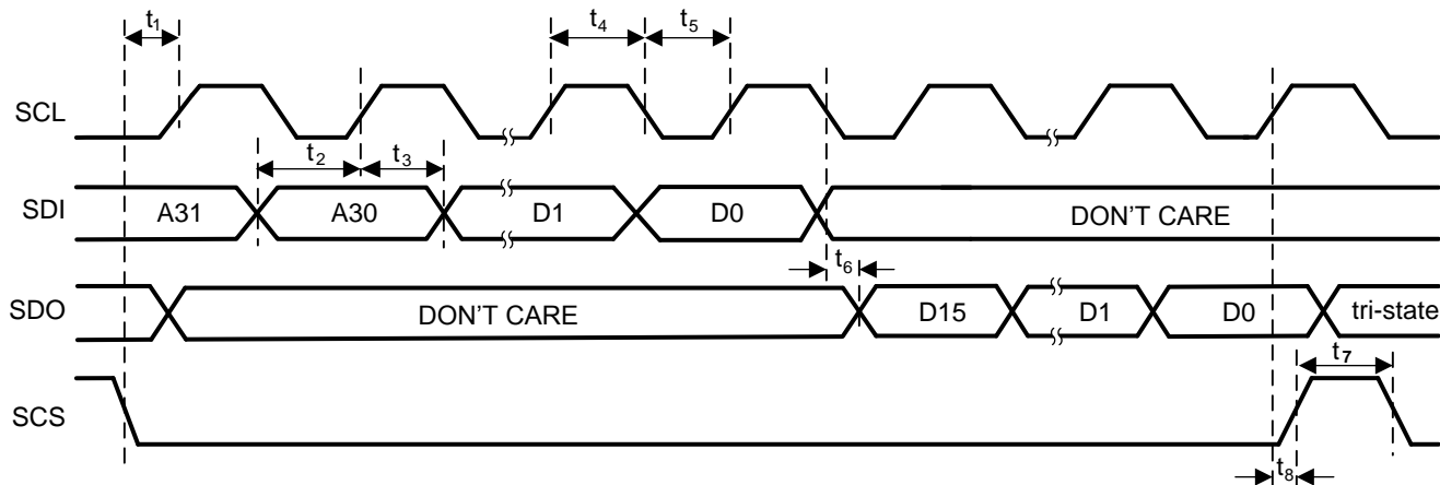
Figure 2. CDCM6208V2G SPI Port Timing
