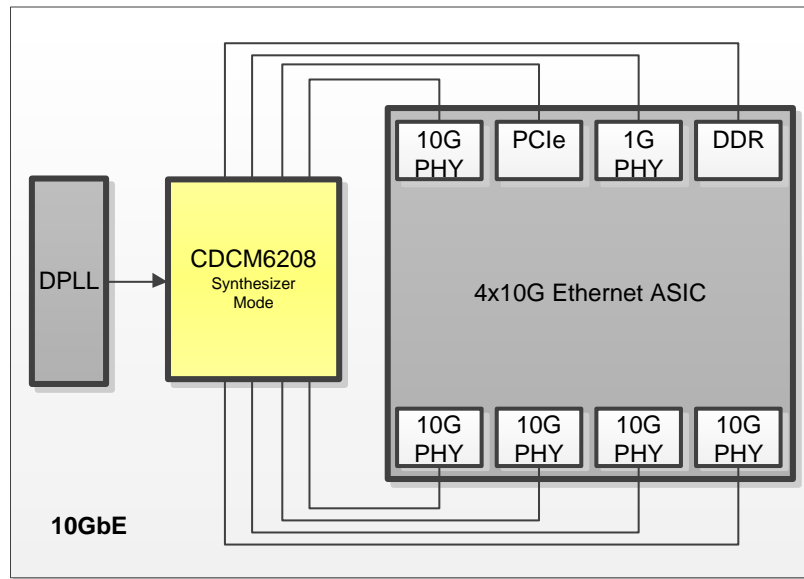
Figure 27. Typical Use Case: CDCM6208V2G Example in Wireless Infrastructure Baseband Application
