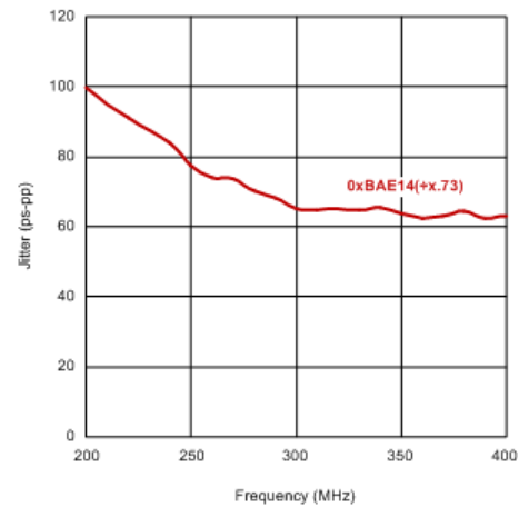
Figure 5. Fractional Divider Input Frequency Impact on Jitter
