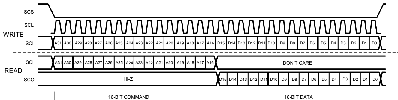
Figure 32. CDCM6208V2G SPI Port Message Sequencing
