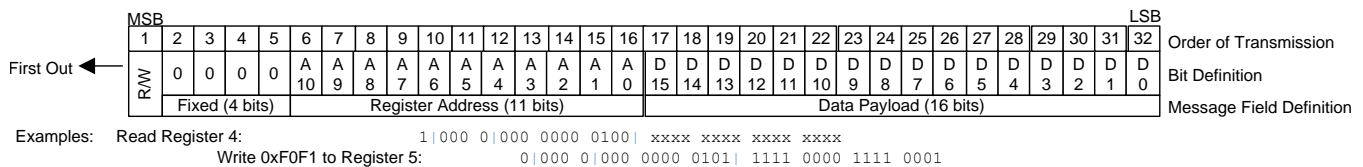
Figure 30. CDCM6208V2G SPI Message Format
