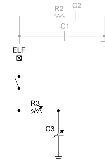
Figure 46. CDCM6208V2G PLL Loop Filter Topology
