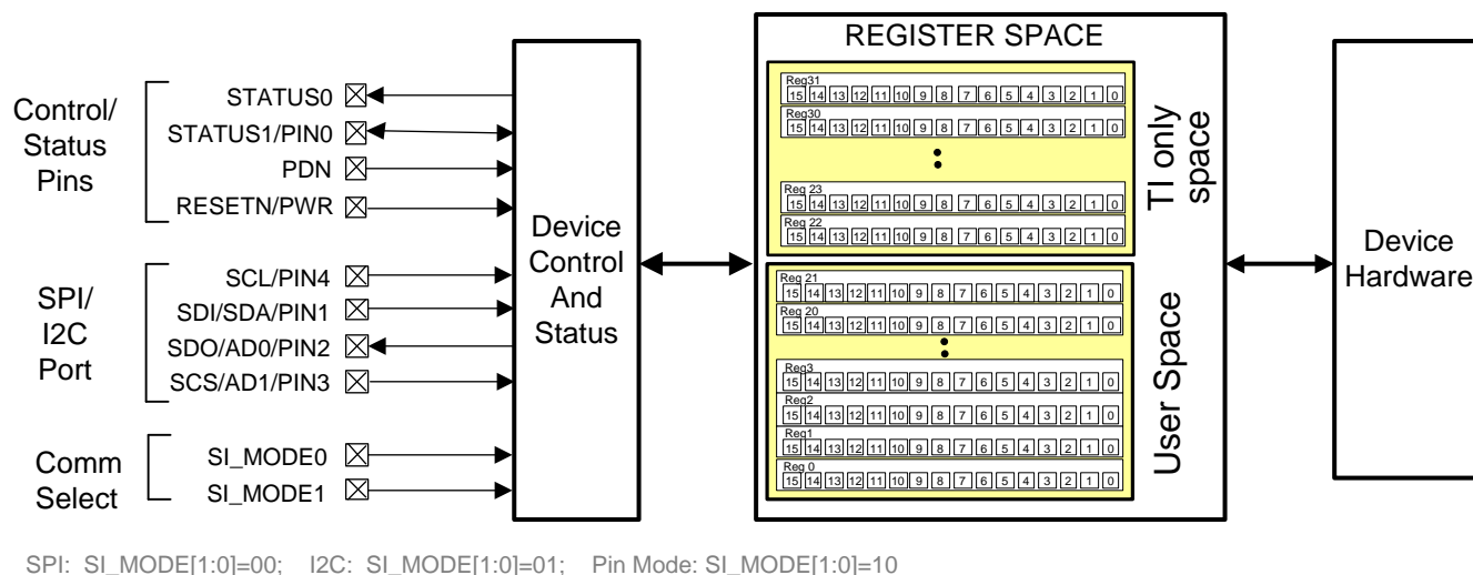
Figure 28. CDCM6208V2G Interface and Control Block
