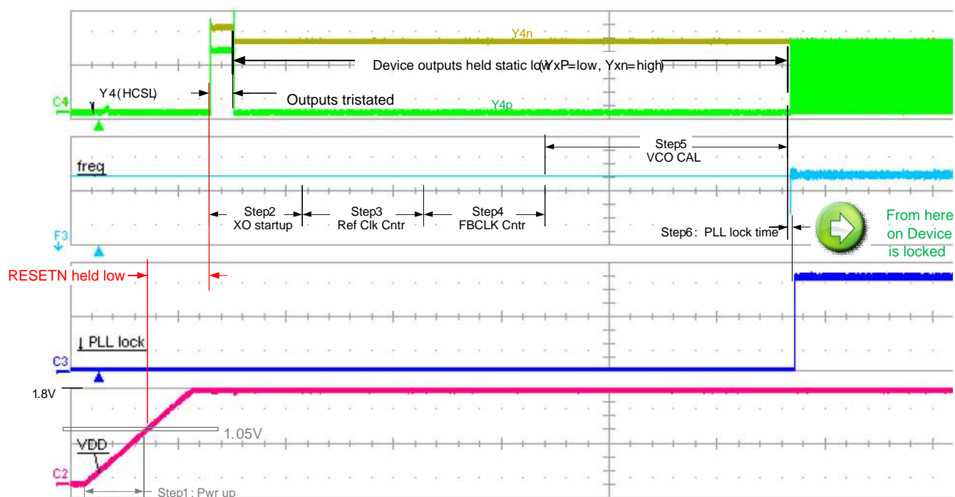
Figure 42. Powerup Time
