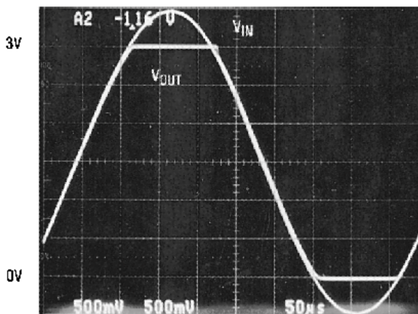
Figure 56. Input Voltage
