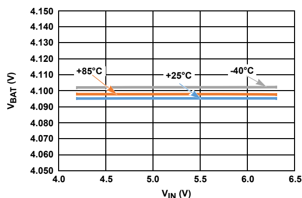
FIGURE 5. NO LOAD VOLTAGE vs TEMPERATURE
