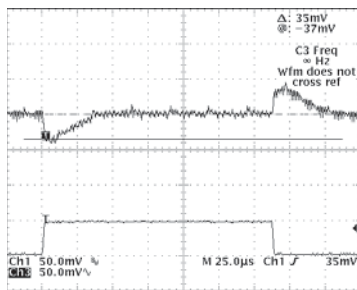
1.8V Transient Response
