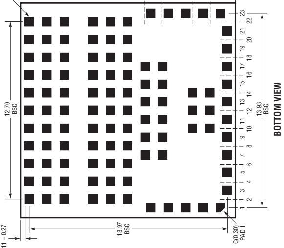
SUGGESTED SOLDER PAD LAYOUT
