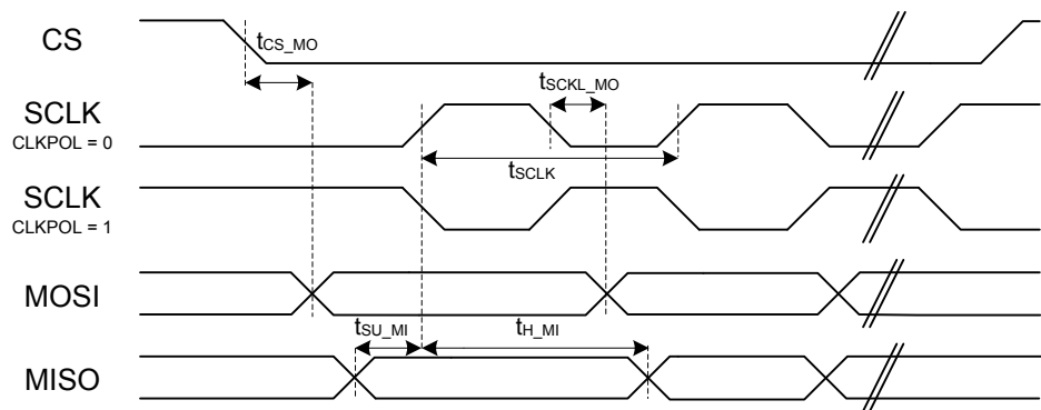
Figure 4.42. SPI Master Timing
