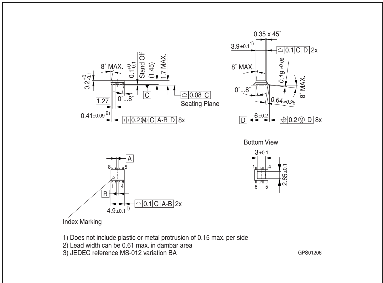
Figure 9 Outline PG-DSO-8
