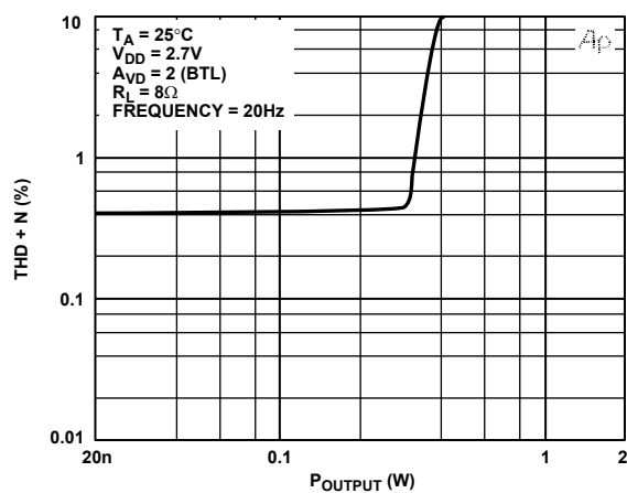
Figure 22. THD + N vs. P_{OUT}
