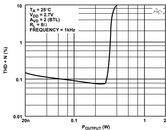
Figure 23. THD + N vs. P_{OUT}
