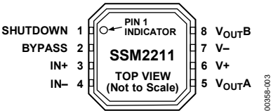
Figure 3. 8-Lead LFCSP_VD Pin Configuration (CP-8-2)
