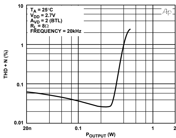
Figure 24. THD + N vs. P_{OUT}
