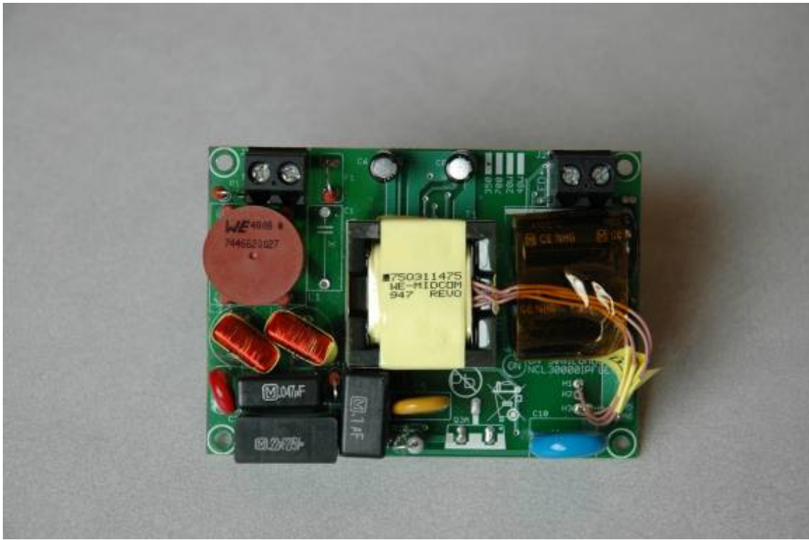
Figure 1. Top Side of Board
