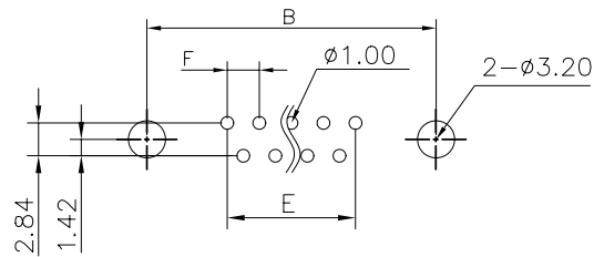
RECOMMENDED P.C.B LAYOUT (TOLERANCE \pm 0.03 )
