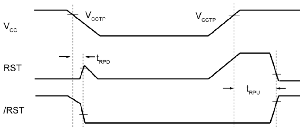
Figure 1. Power-Up/Power-Down Sequence
