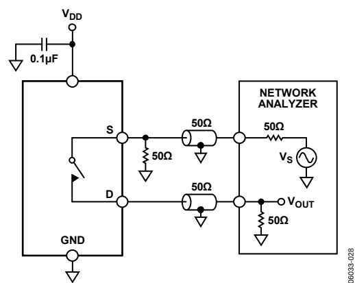
Figure 26. Off Isolation
