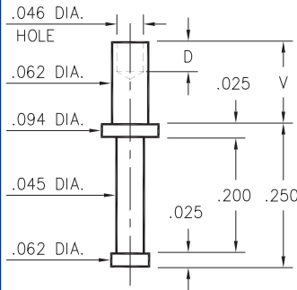
2329-X-00-XX-00-00-07-0 Swage mount in .067 hole
