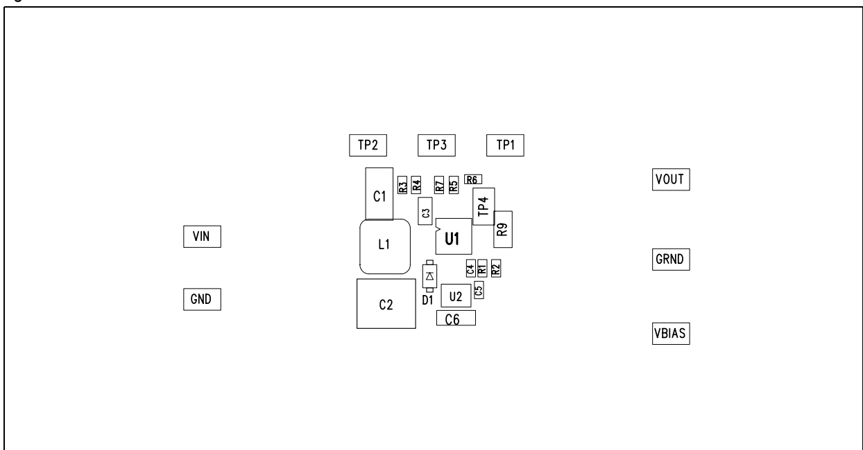
Figure 5. Placement TOP
