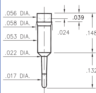
0952-0-00-XX-00-00-03-0 Press-fit in .056 mounting hole
