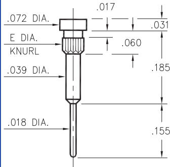
1067-X-00-XX-00-00-03-0 Press-fit in .042/.055 mounting hole
