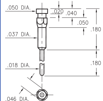
0522-0-00-XX-00-00-03-0 Pentagonal press-fit in .042 plated thru hole
