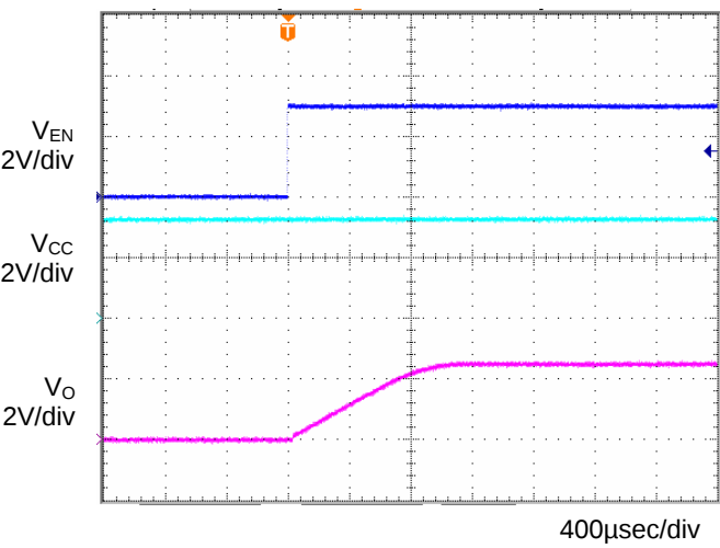
Fig.15 Input sequence 2 Co=1 \mu F, Ta=-40 ^{\circ} C
