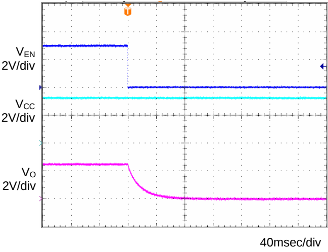
Fig.18 OFF sequence 2 Co=1 \mu F, Ta=-40 ^{\circ} C
