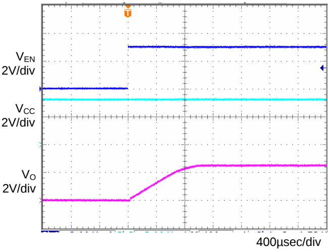
Fig.16 Input sequence 2 Co=1 \mu F, Ta=25 ^{\circ} C
