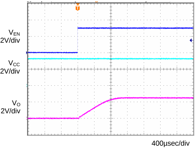
Fig.17 Input sequence 2 Co=1 \mu F, Ta=105 ^{\circ} C
