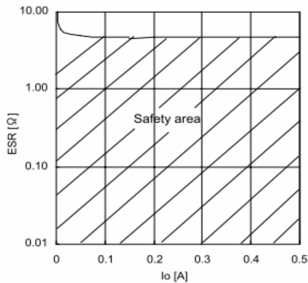
Fig.31 ESR safety area
