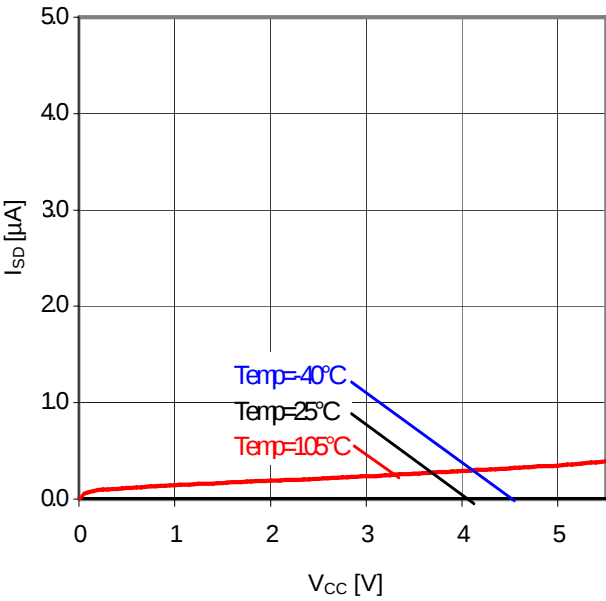
Fig.26 V_{CC} - I_{SD} ( V_{EN}=0\text{V} )
