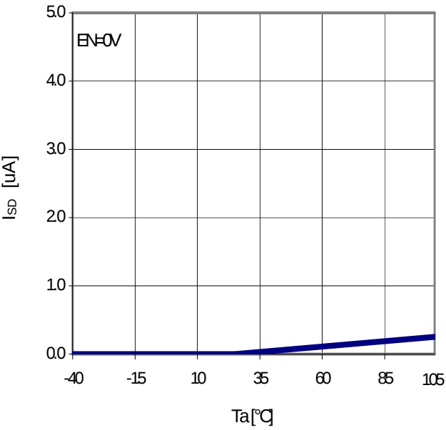
Fig.23 T_a - I_{SD} ( V_{EN}=0\text{V} )
