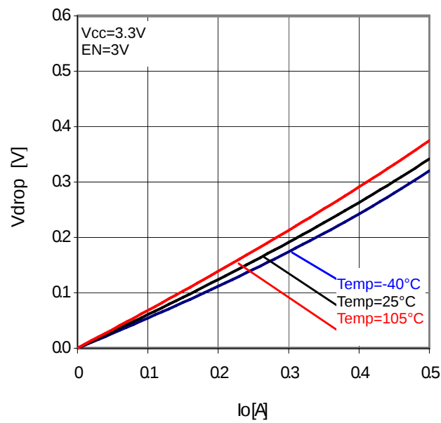
Fig.35 Minimum dropout Voltage 2 (VCC=3.3V)
