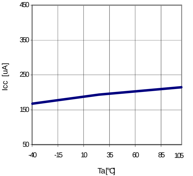
Fig.22 T_a - I_{CC}
