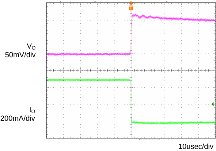
Fig.7 Transient Response (0.5→0A) Co=1μF,Ta=25°C
