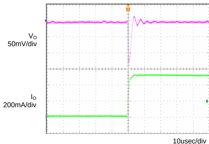
Fig.3 Transient Response (0→0.5A) C_o=1\mu F , T_a=-40^\circ C
