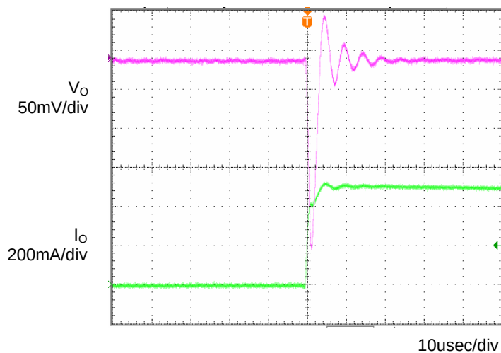
Fig.5 Transient Response (0→0.5A) C_o=1\mu F , T_a=105^\circ C
