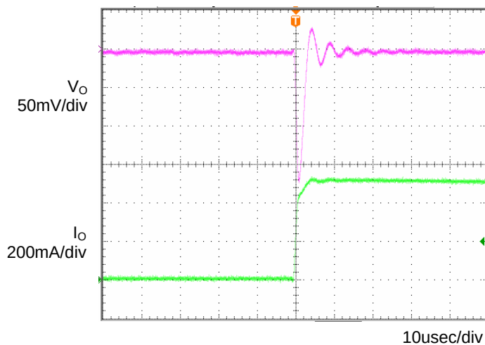
Fig.4 Transient Response (0→0.5A) C_o=1\mu F , T_a=25^\circ C
