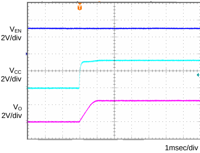
Fig.10 Input sequence 1 Co=1µF,Ta=25°C
