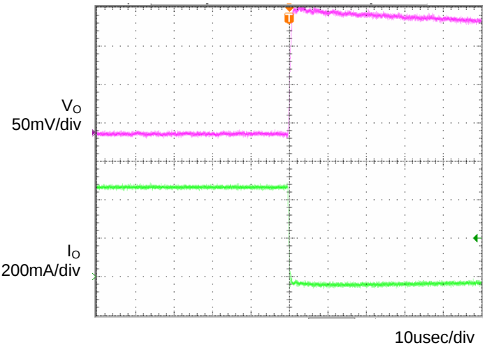
Fig.8 Transient Response (0.5→0A) Co=1µF,Ta=105°C
