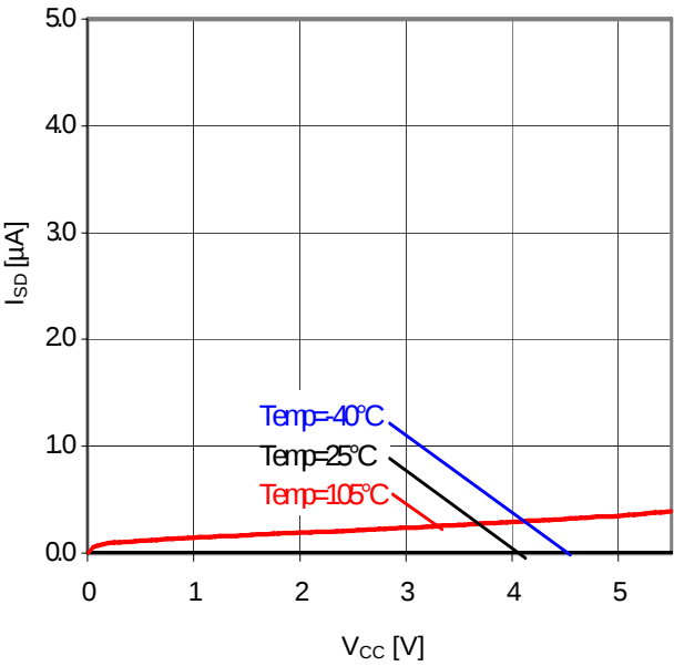
Fig.26 V_{CC} - I_{SD} ( V_{EN}=0V )
