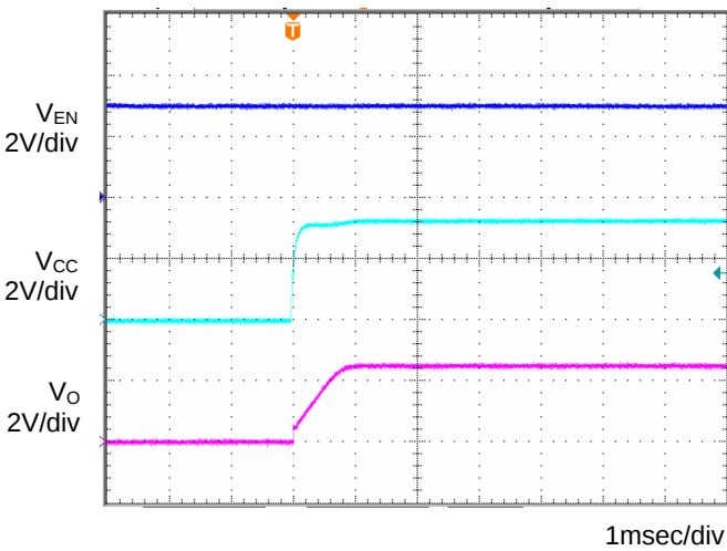
Fig.9 Input sequence 1 Co=1µF,Ta=-40°C
