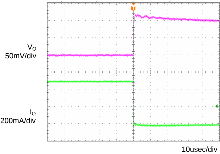
Fig.7 Transient Response (0.5→0A) Co=1µF,Ta=25°C
