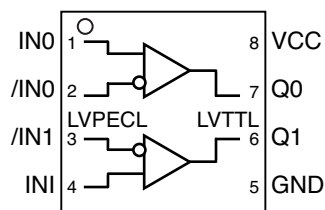
8-Pin MLF®
