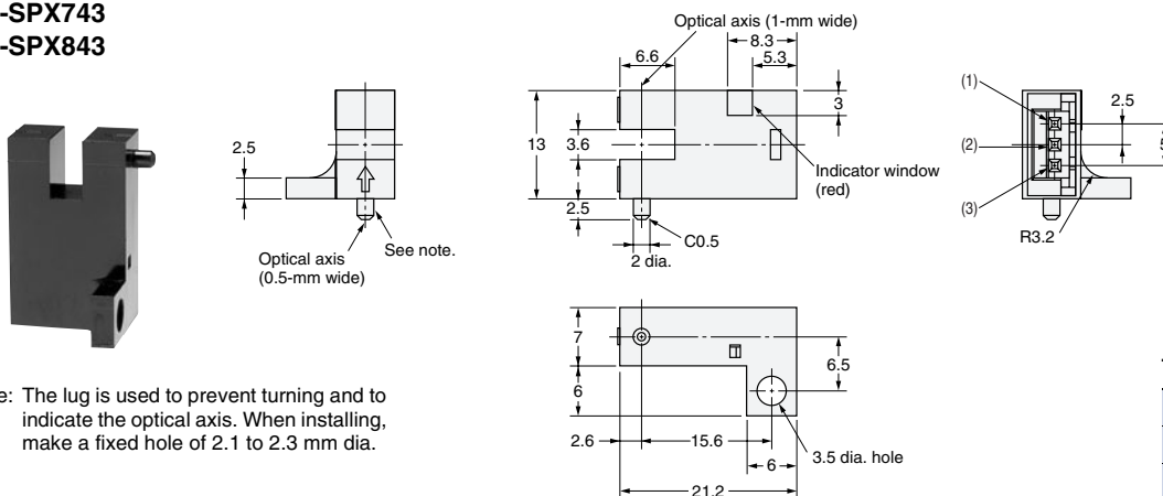
Terminal Arrangement
