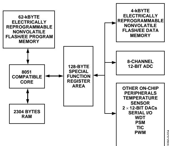
Figure 26. Programming Model
