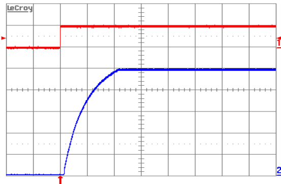
Figure 7. Turn-on transient at full rated load current (resistive) plus 10,000 \mu\text{F} at V_{\text{in}} = 48\text{ V} , triggered via ON/OFF pin. Top trace: ON/OFF signal (5 V/div.). Bottom trace: Output voltage (1 V/div.). Time scale: 5 ms/div.
