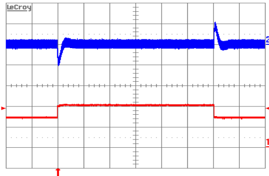
Figure 9. Output voltage response to load current step-change (6.5 A–9.75 A–6.5 A) at V_{\text{in}} = 48\text{ V} . Top trace: output voltage (100 mV/div.). Bottom trace: load current (5 A/div.). Current slew rate: 5 A/ \mu\text{s} . C_o = 470\mu\text{F} POS + 1 \mu\text{F} ceramic. Time scale: 0.2 ms/div.
