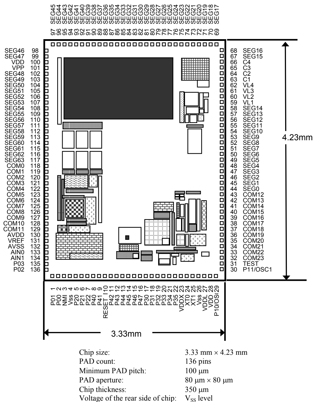
Figure 6 ML610Q436 Chip Layout &amp; Dimension
