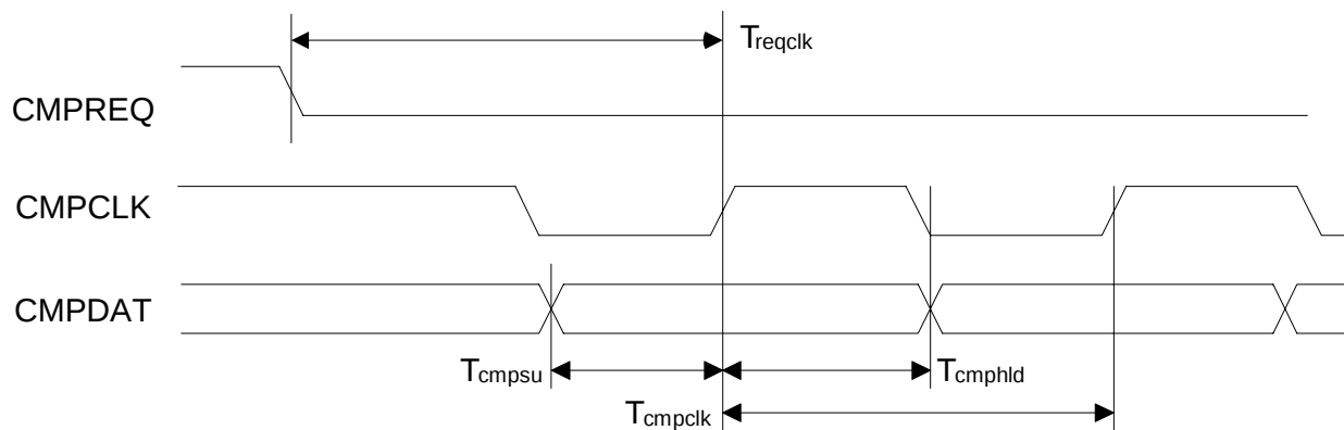
Figure 10. Serial Compressed Data Timing
