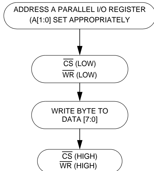
Figure 24. Intel Mode, One-Byte Write Flow Dia-
