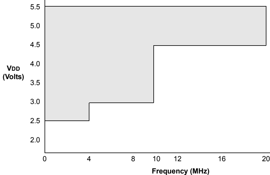
FIGURE 12-2: PIC16F676 WITH A/D ENABLED VOLTAGE-FREQUENCY GRAPH, -40^{\circ}\text{C} \leq T_A \leq +125^{\circ}\text{C}
