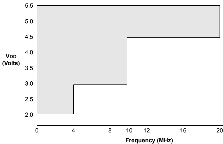
FIGURE 12-1: PIC16F630/676 WITH A/D DISABLED VOLTAGE-FREQUENCY GRAPH, -40^{\circ}\text{C} \leq T_A \leq +125^{\circ}\text{C}
