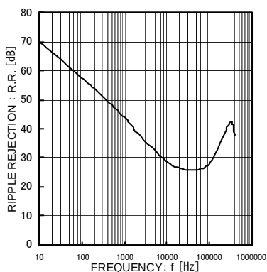
Fig.19 Ripple Rejection ( I_o=100\text{mA} )
