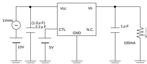
Measurement Circuit of Fig.7 and Fig.19
