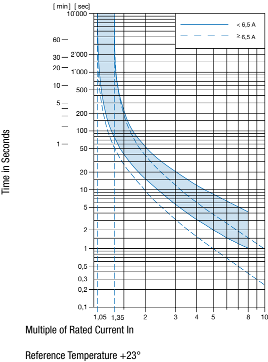
Time-Current-Curves
