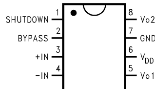
Figure 2. Top View See Package Number D or P
