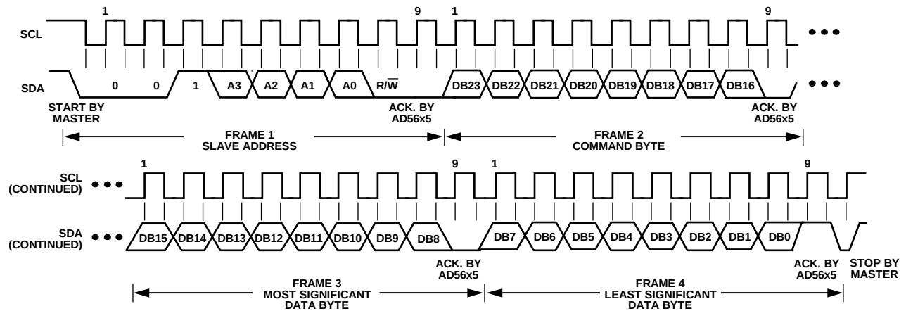
Figure 59. I 2 C Write Operation (14-Lead Package)
