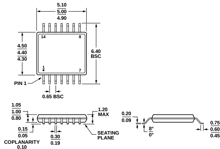
COMPLIANT TO JEDEC STANDARDS MO-153-AB-1 Figure 76. 14-Lead Thin Shrink Small Outline Package [TSSOP] (RU-14)
