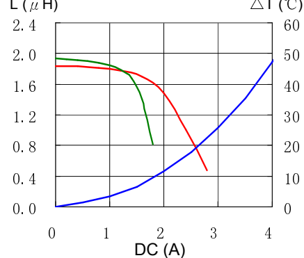
5. CDRH4D22NP-3R9NC
