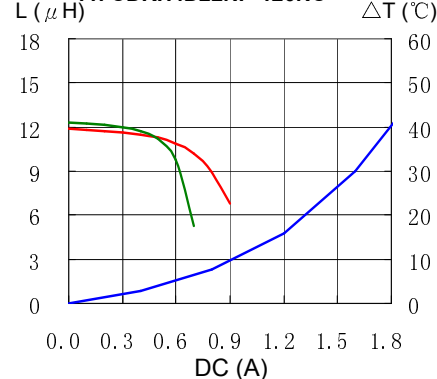
11. CDRH4D22NP-120NC
