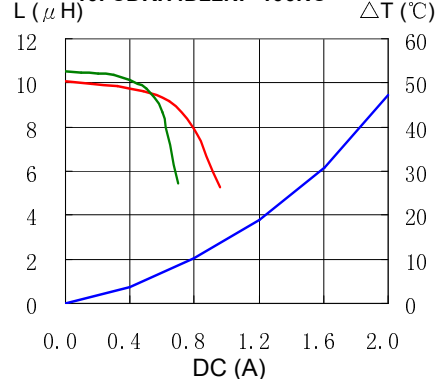
10. CDRH4D22NP-100NC
