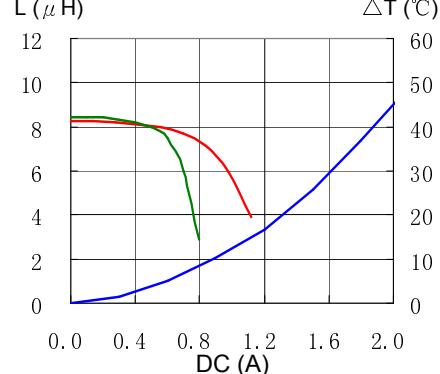
12. CDRH4D22NP-150NC
