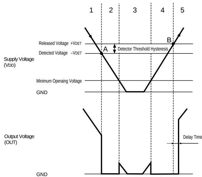
FIG. 2 Operation Diagram
