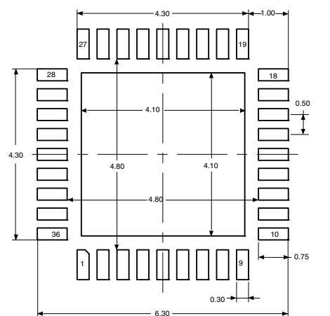
Figure 42. Recommended footprint (dimensions in mm) (1)(2)
