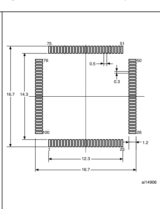
Figure 48. Recommended footprint (1)(2)
