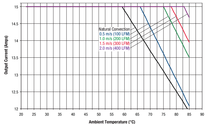
Maximum Current Temperature Derating @ sea level ( V_{in} = 48\text{ V} , transverse airflow, with baseplate)
