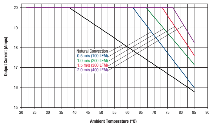
Maximum Current Temperature Derating @ sea level (Vin = 24V, transverse airflow, no baseplate)
