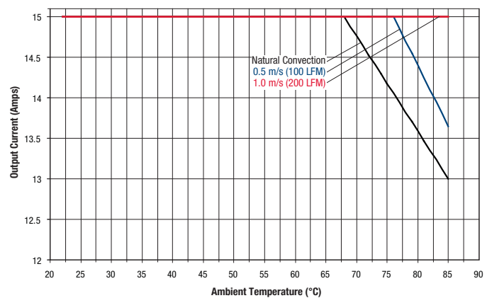
Maximum Current Temperature Derating @ sea level ( V_{in} = 24\text{ V} , transverse airflow, with baseplate)
