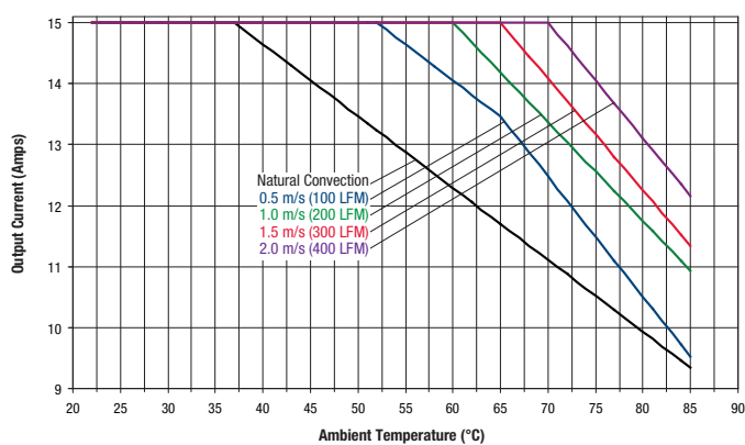
Maximum Current Temperature Derating @ sea level ( V_{in} = 48\text{ V} , transverse airflow, no baseplate)
