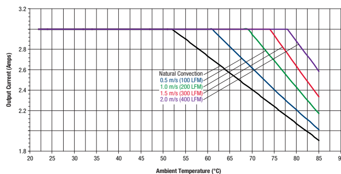
Maximum Current Temperature Derating @sea level (Vin = 24V, transverse airflow, with baseplate)
