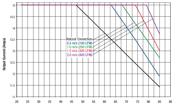
Maximum Current Temperature Derating @ sea level ( V_{in} = 24\text{ V} , transverse airflow, no baseplate)
