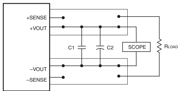
C1 = 0.47µF CERAMIC C2 = NA LOAD 2-3 INCHES (51-76mm) FROM MODULE
