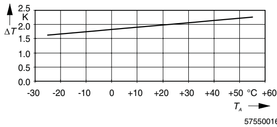
Figure 11 Systematic temperature measuring error \Delta T depending on the cable temperature T_A
