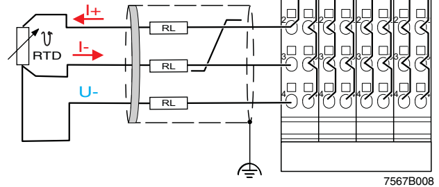
Figure 5 3-wire termination example
