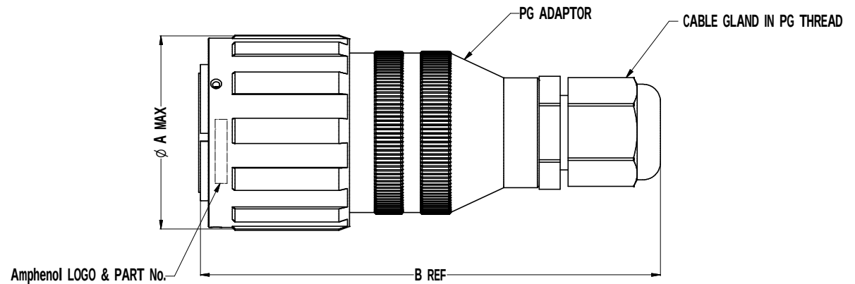
85 AND 150 CONTACT TYPE
