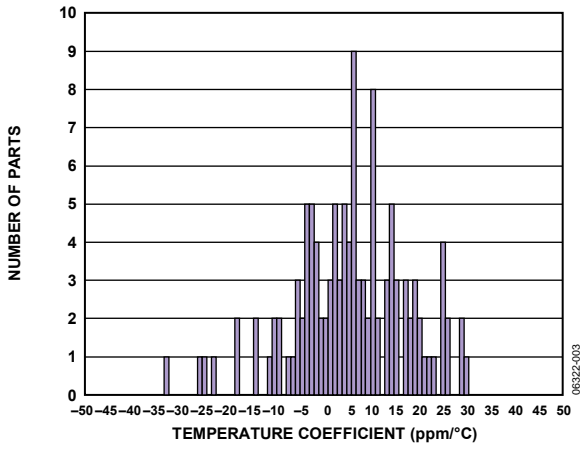
Figure 3. Temperature Coefficient, V_{OUT} = 0.5 V
