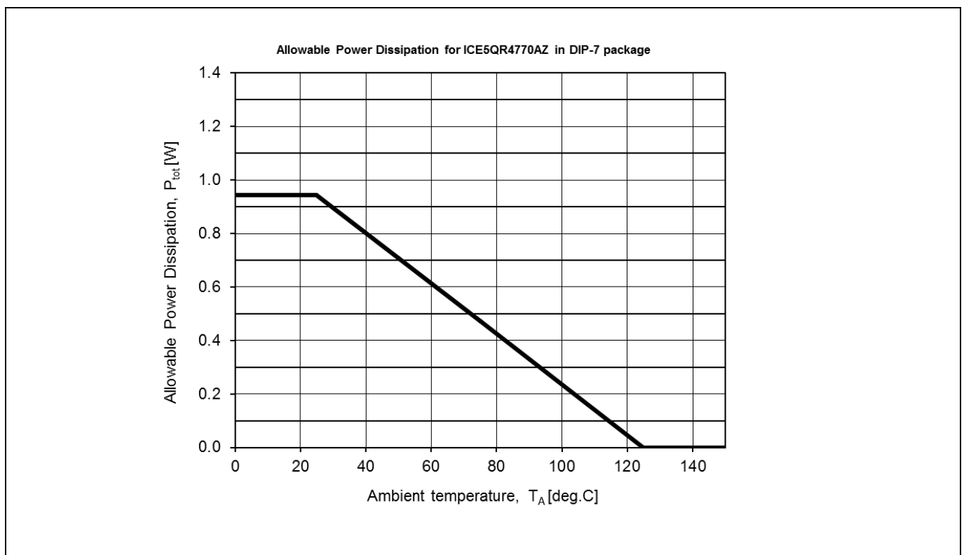
Figure 23 Power dissipation of ICE5QR4770AZ, DIP-7 package; P_{\text{tot}} = f(T_a) , (Maximum ratings as given in section 4.1 must not be exceeded)
