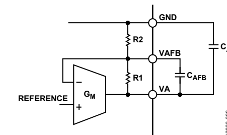
Figure 47. C_A and C_{\text{AFB}} Connection to the G_M Amplifier
