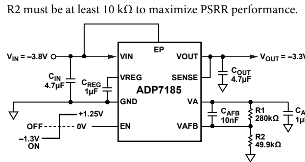
Figure 42. Setting the Adjustable Output Voltage
