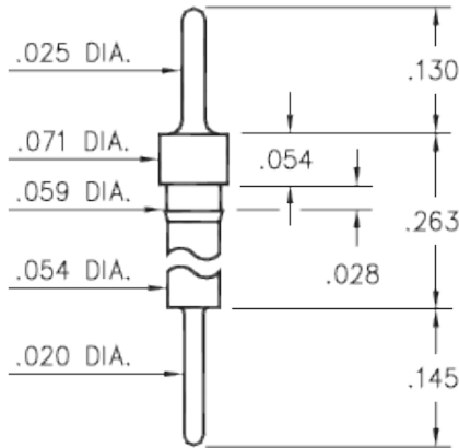
8859-0-00-XX-00-00-03-0 Press-fit in .056 mounting hole
