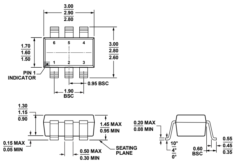
COMPLIANT TO JEDEC STANDARDS MO-178-AB Figure 45. 6-Lead Small Outline Transistor Package (SOT-23) (RJ-6) Dimensions shown in millimeters
