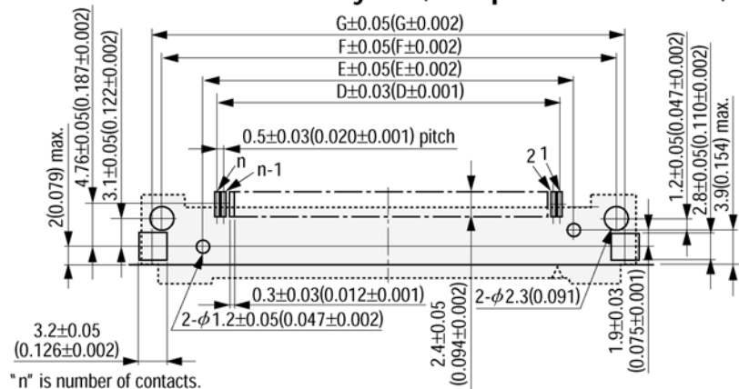
Printed Circuit Board Layout (Component Side View)
