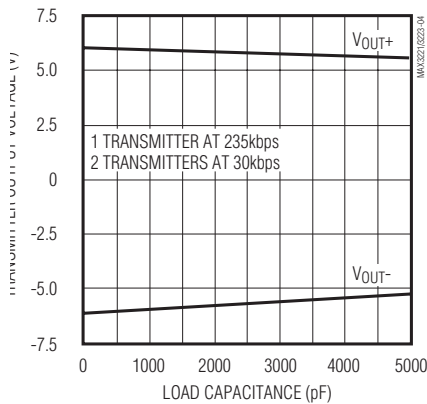
MAX3243 TRANSMITTER OUTPUT VOLTAGE vs. LOAD CAPACITANCE
