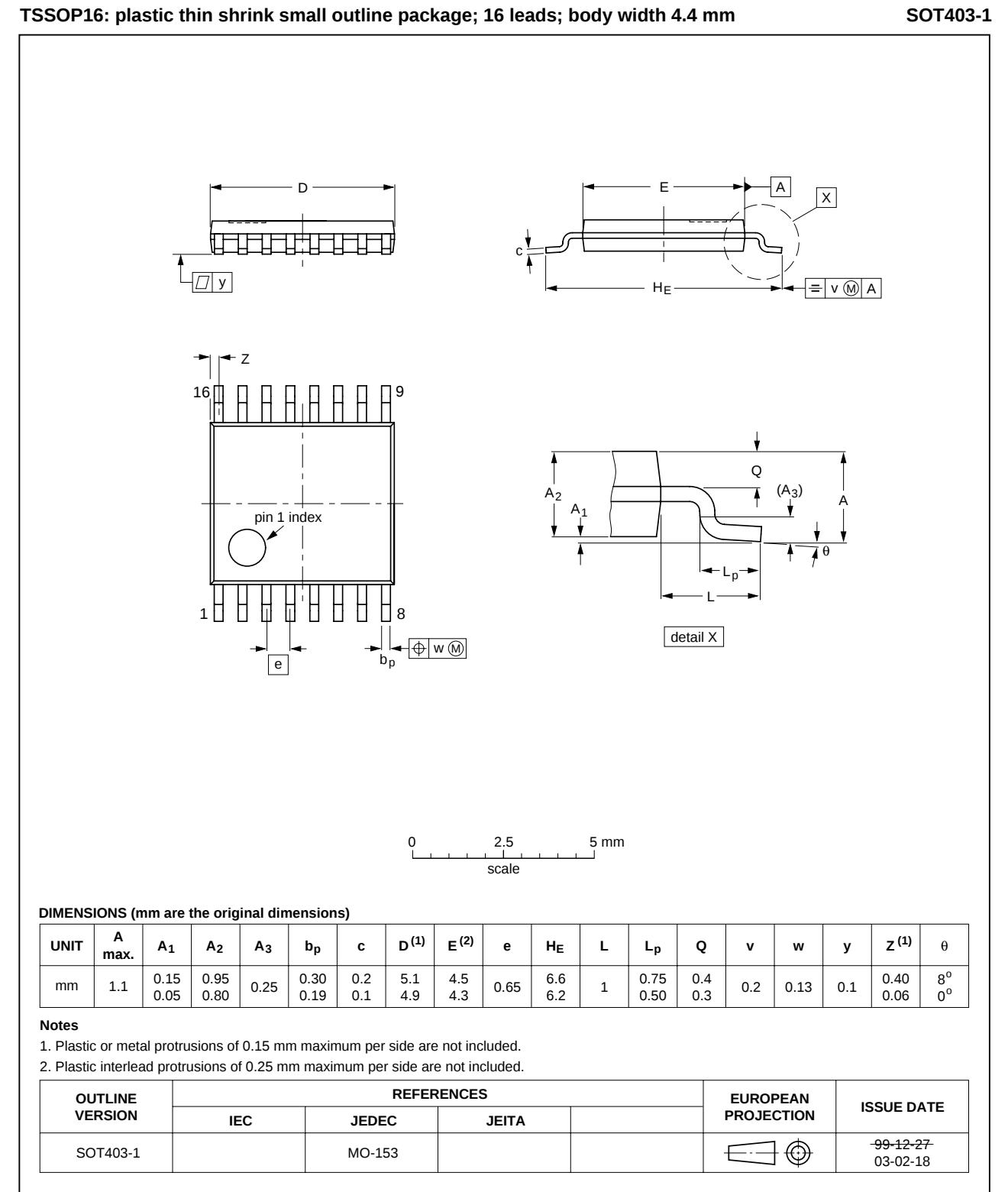
Fig 25. Package outline SOT403-1 (TSSOP16)
