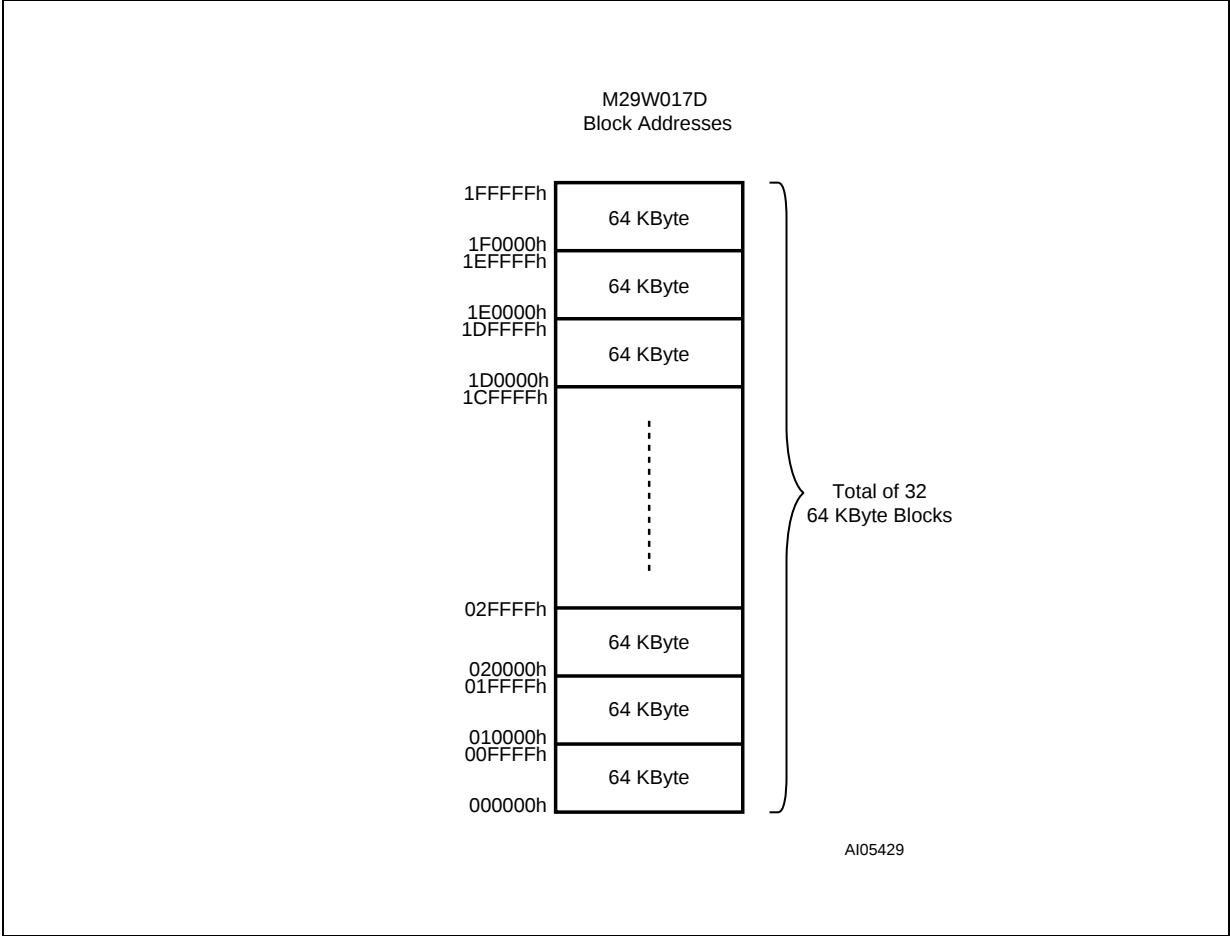
Figure 5. Block Addresses
