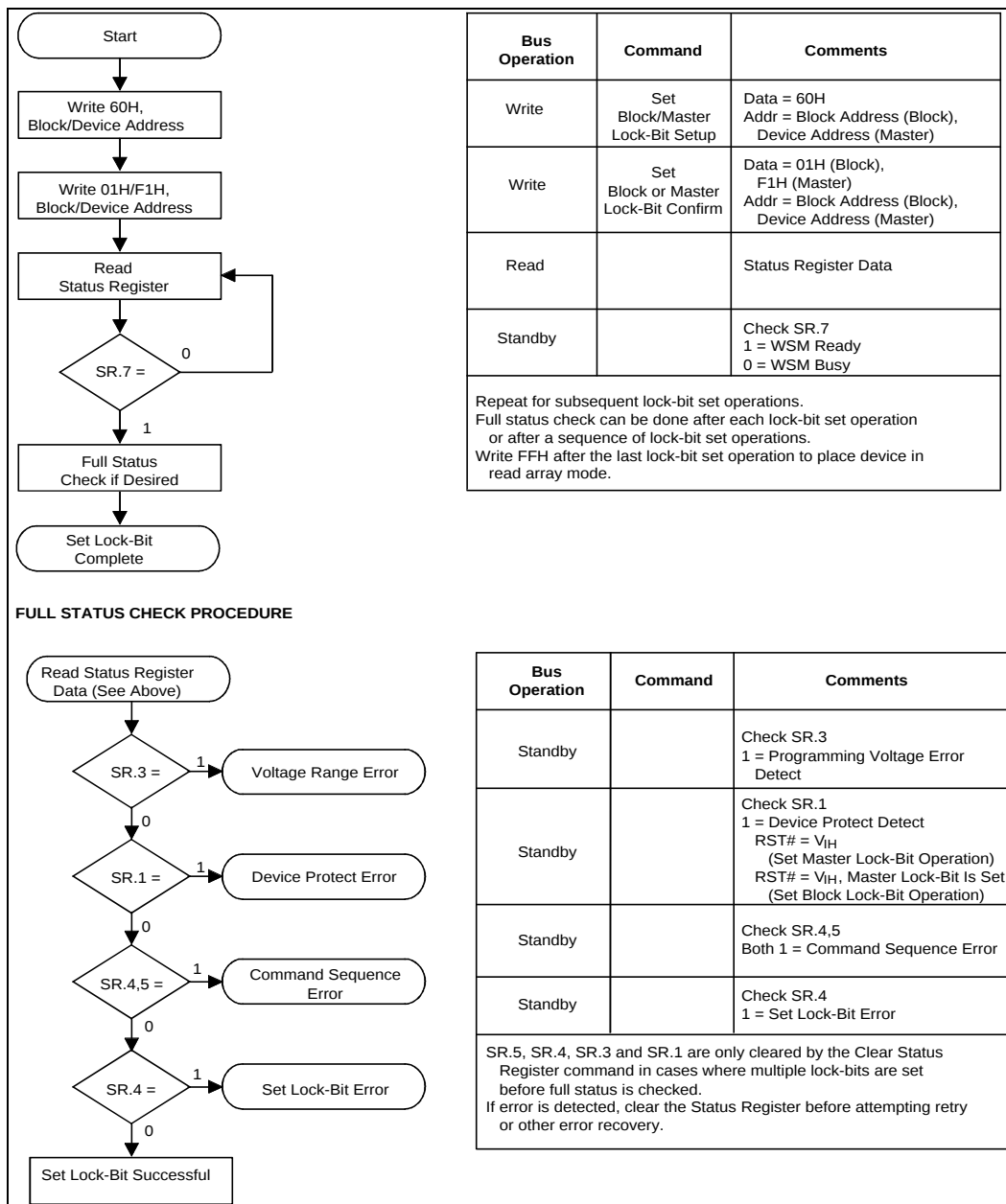
Figure 12. Set Block Lock-Bit Flowchart
